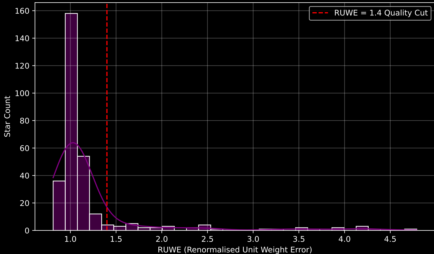
GAPOGEE DR17 Field [059+36_MGA] RUWE Distribution (n= 298)
