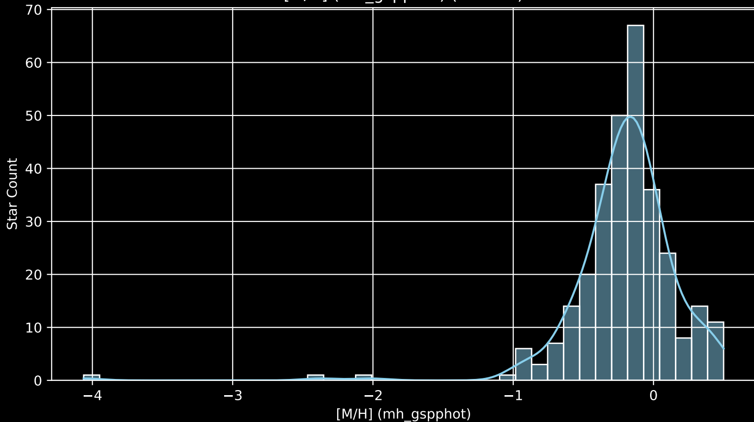
APOGEE DR17 Field: [059+36_MGA [M/H] (mh_gspphot) (n= 301)
