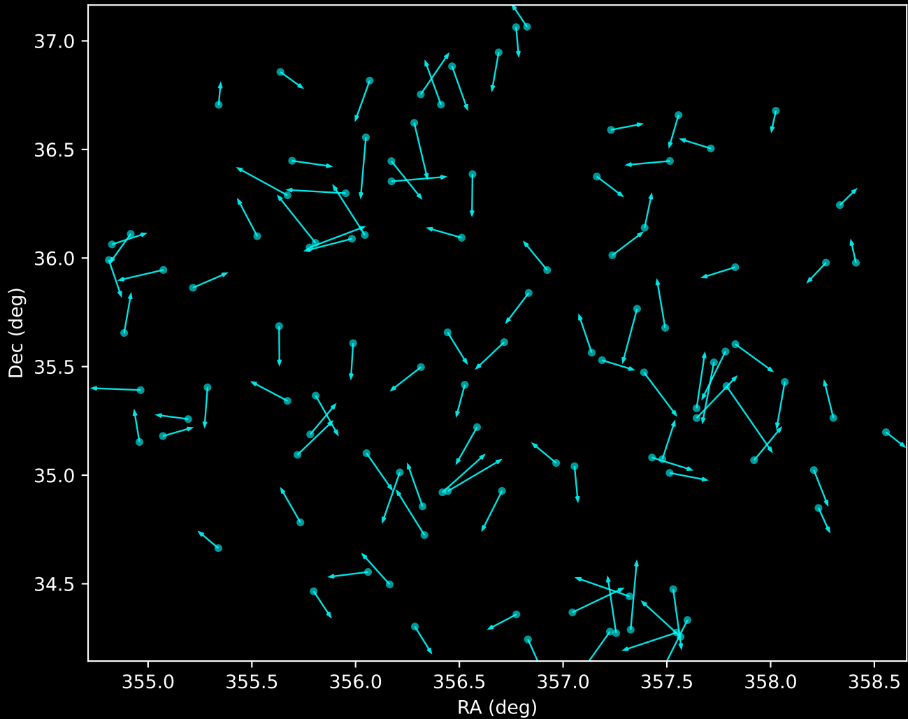
APOGEE DR17 Noise Stream Proper Motion Vectors (n=105)
