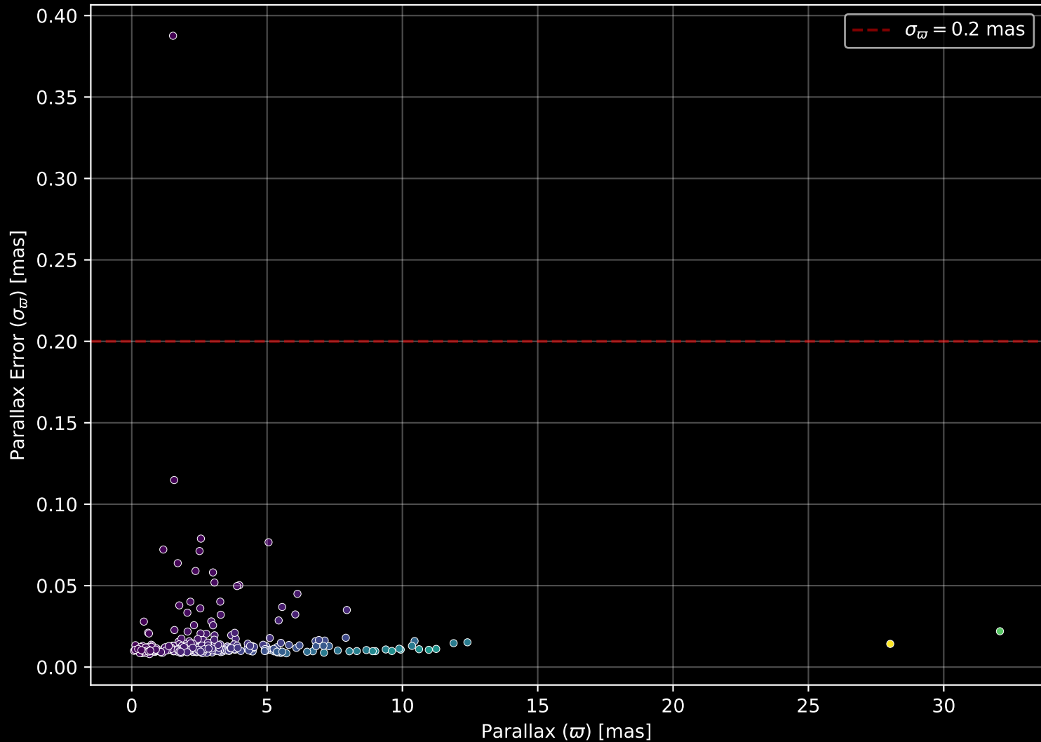
APOGEE DR17 Field: [059+36_MGA] Parallax Quality (n= 306)
