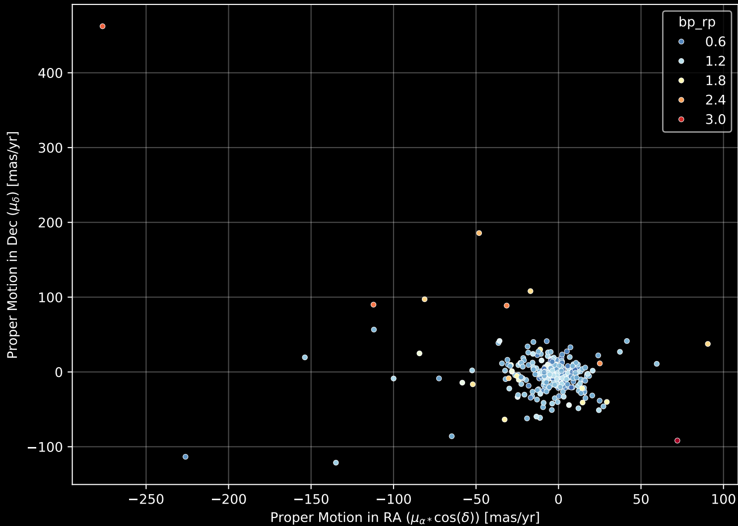
APOGEE DR17 Field: [059+36_MGA] Proper Motion Diagram (n= 306)
