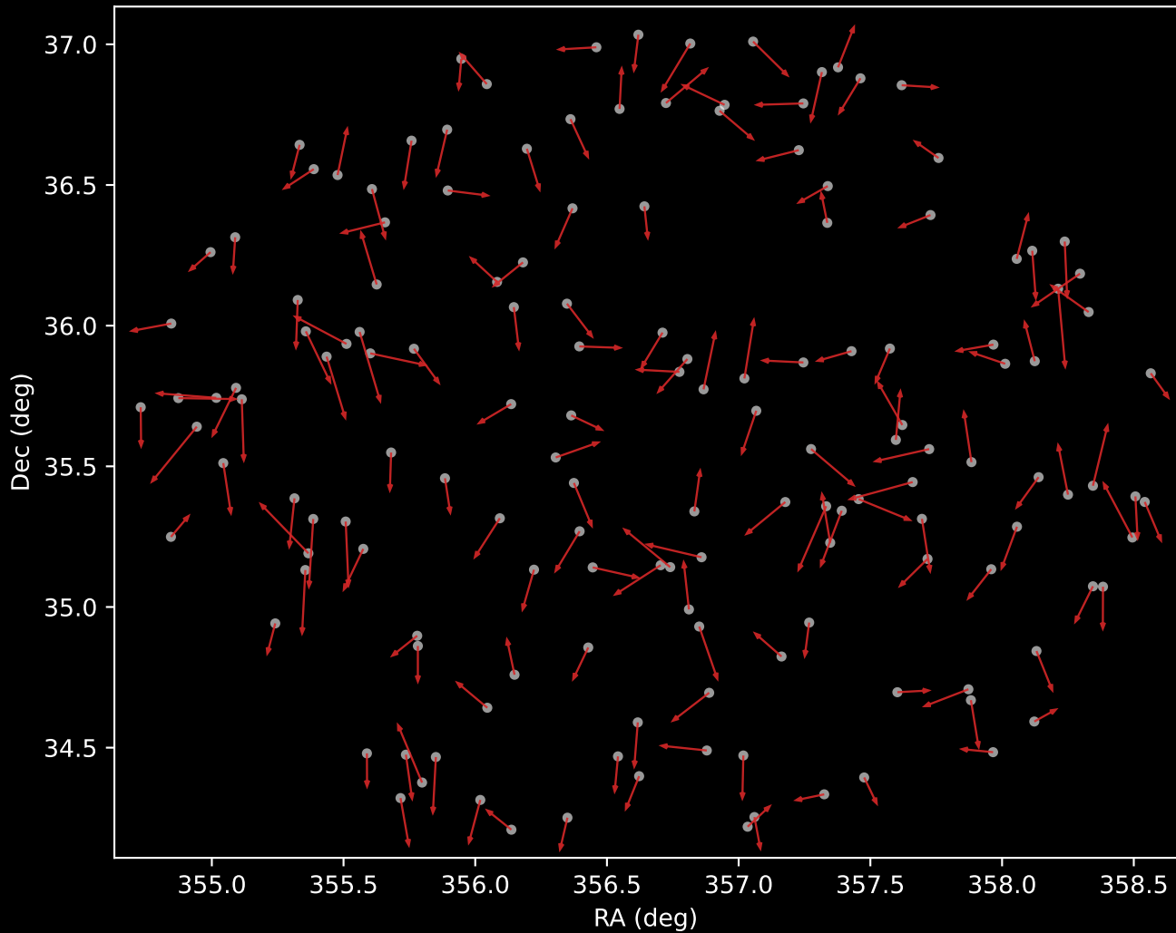
APOGEE DR17 Cluster 6 Proper Motion Vectors (n=152)
