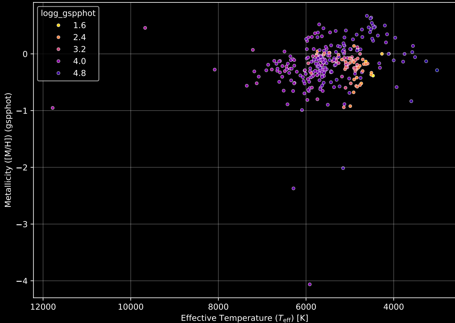
APOGEE DR17 Field: [059+36_MGA] Stellar Population Parameters (n= 306)
