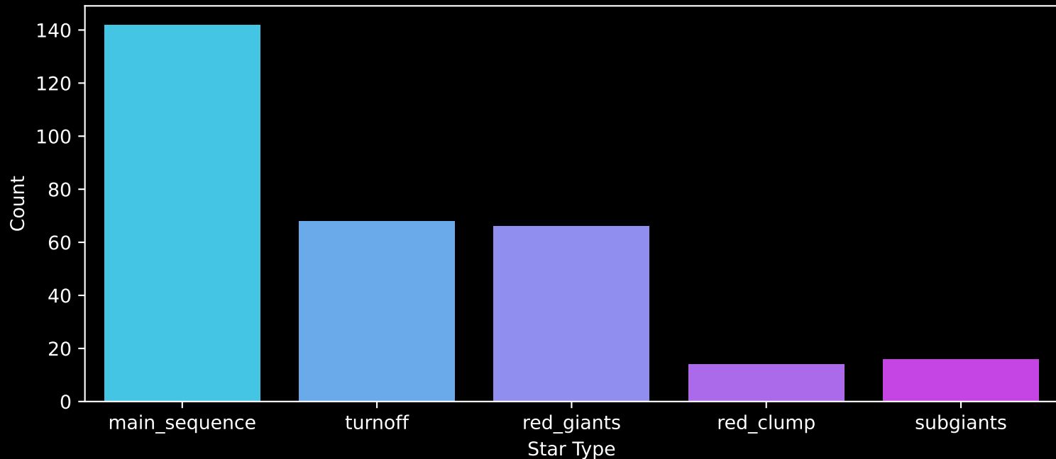
APOGEE DR17 Field: [059+36_MGA] Count plot of Star Type
